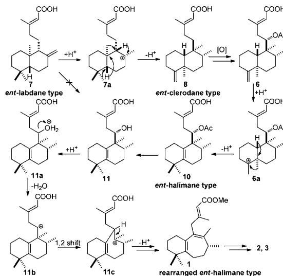
Scheme 1. Plausible Biogenetic Pathway of the ent -Halimane and 10(9→11) abeo - ent -Halimane Diterpenoids in This Plant
