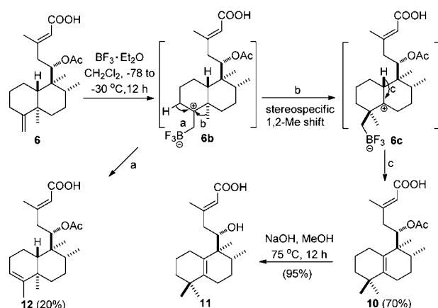
Scheme 2. Synthesis of ent -Halimane Diterpenoid 11 from 6
